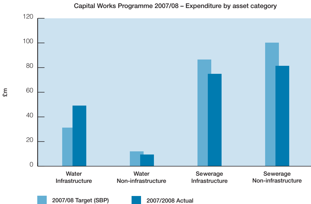
Figure 5: Capital Works Programme expenditure by asset category
