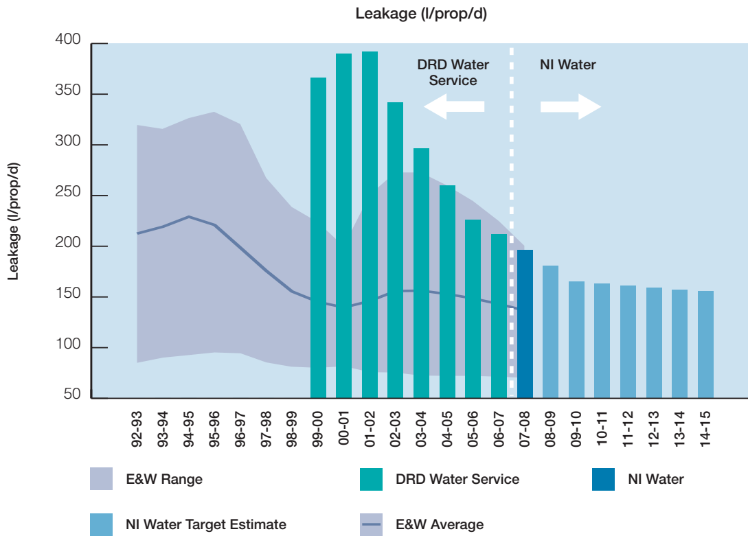
Figure 13: NI Water average daily leakage per property
