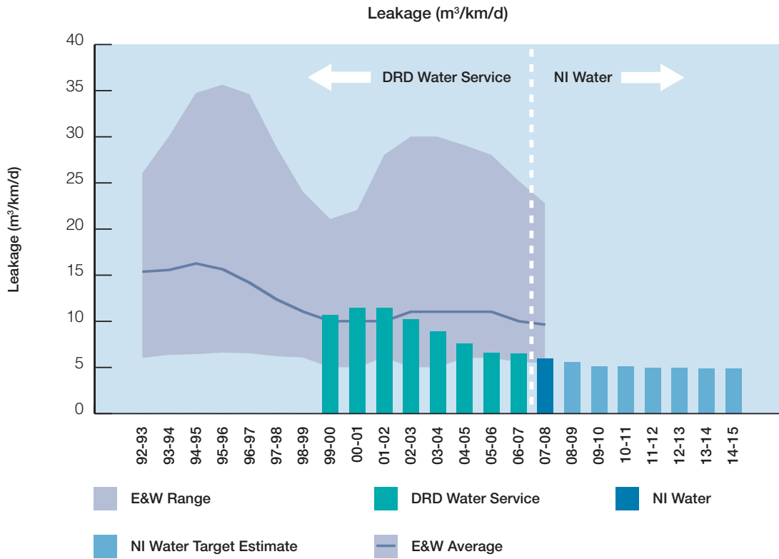
Figure 12: NI Water average daily leakage per km of water pipe
