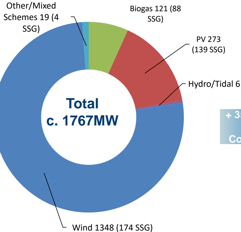
NI Connected Renewable Generation Technology Mix
