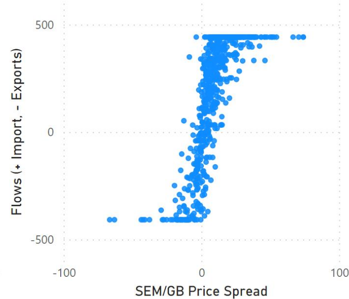
Moyle Flows vs SEM/GB Price Spread
