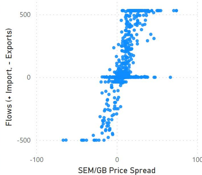
EWIC Flows vs SEM/GB Price Spread
