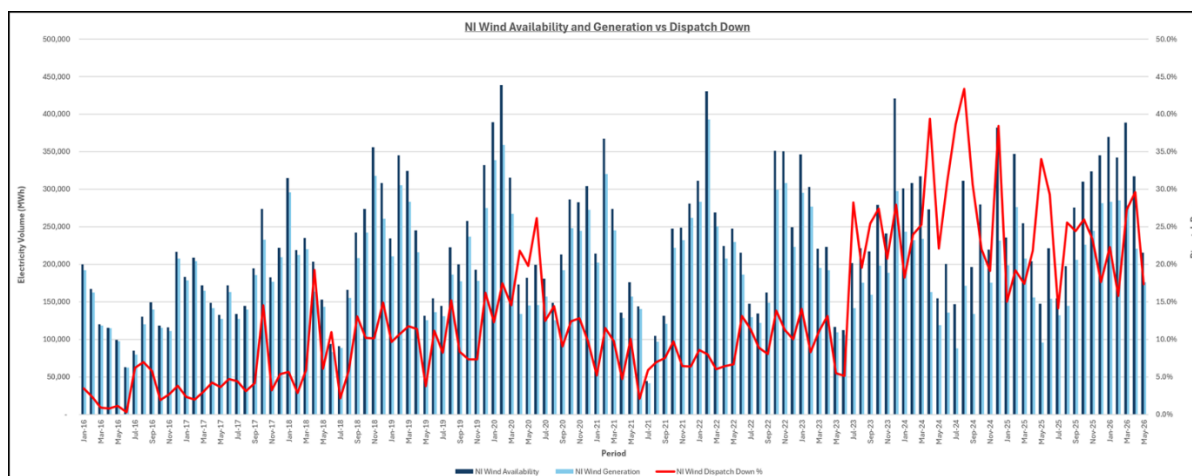
Figure 1 - Wind Availability, Generation and Dispatch Down Rates in Northern Ireland, 2016 to 2026 13
