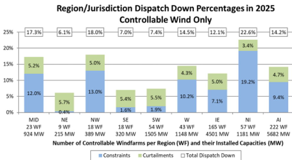
Figure 2 - All-Island Dispatch Down Percentages by Region (2025)
