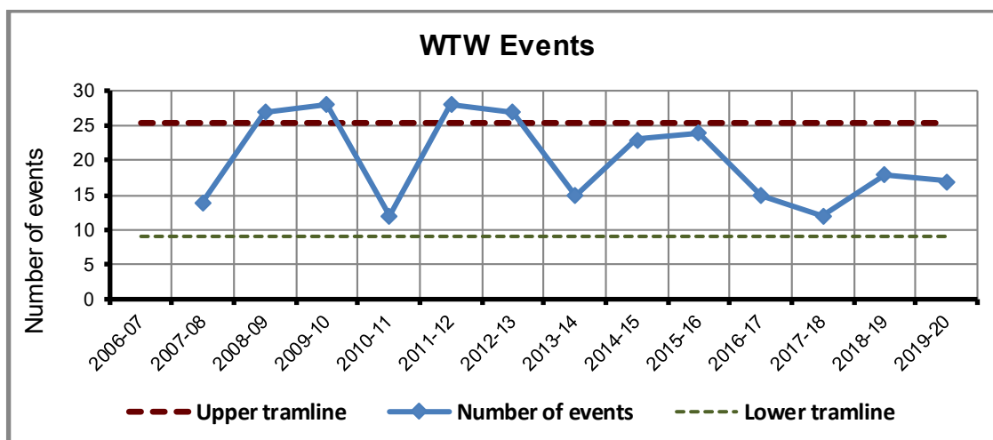
Figure 6.9: Water non-infra - water treatment works events.
