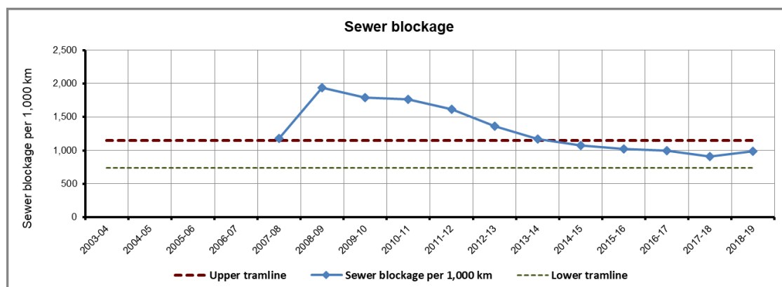
Figure 6.12: Sewerage infra – sewer blockage.
