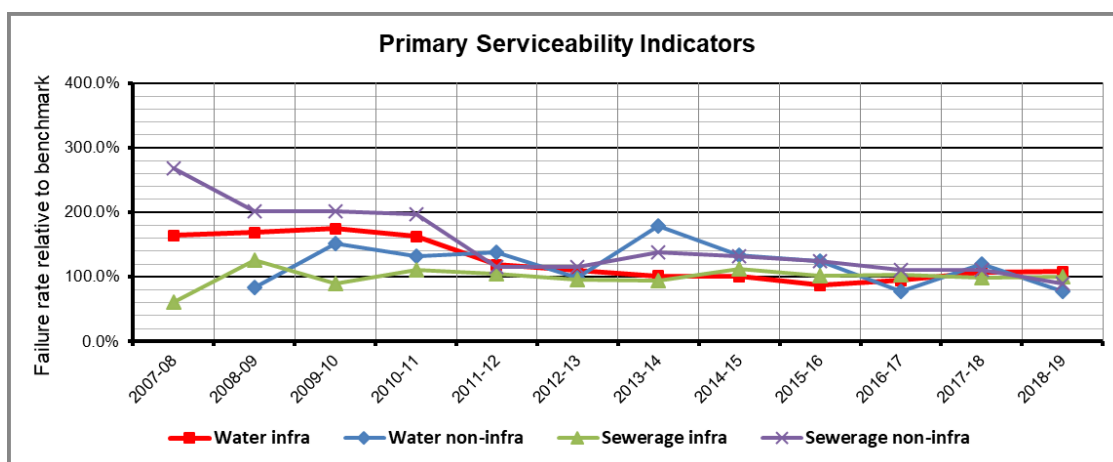
Figure 5.5: Primary serviceability indicators.
