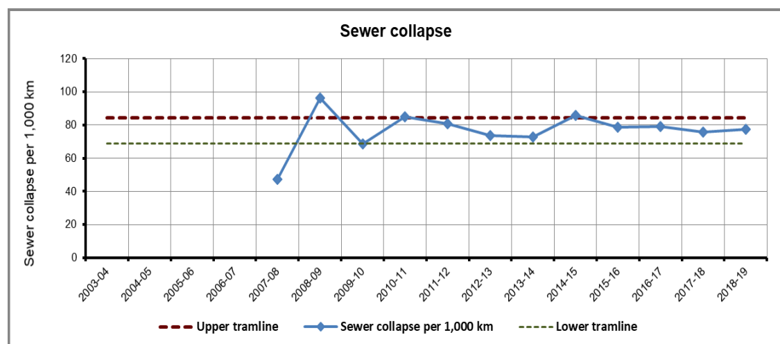
Figure 6.11: Sewerage infra – sewer collapse.
