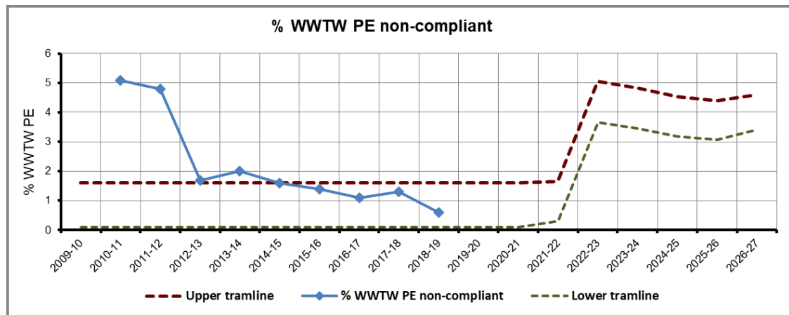
Figure 6.17: Sewerage non-infra - WwTW compliance – population equivalent.
