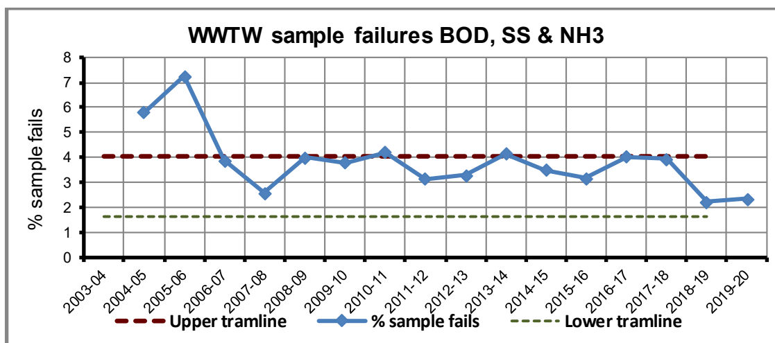
Figure 6.18: Sewerage non-infra - WwTW compliance – samples.
